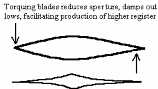
Rotary Torquing
